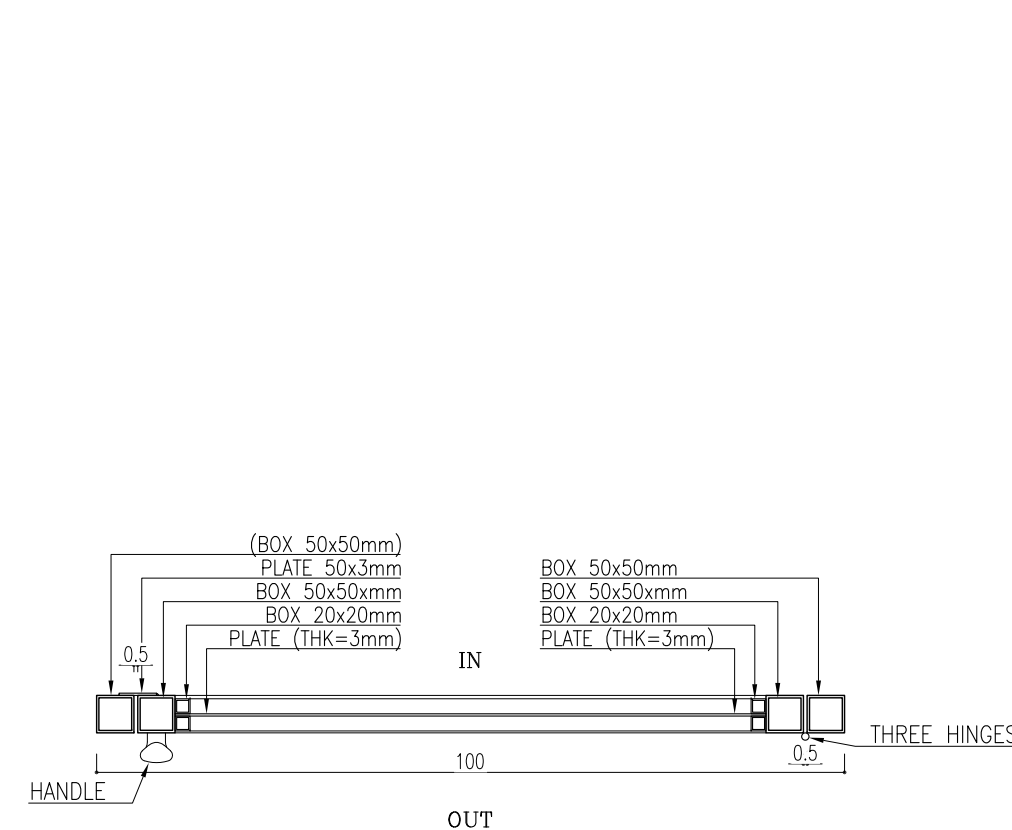
SECTION E-E
