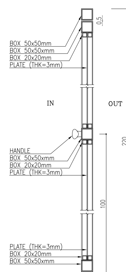
SECTION F-F
