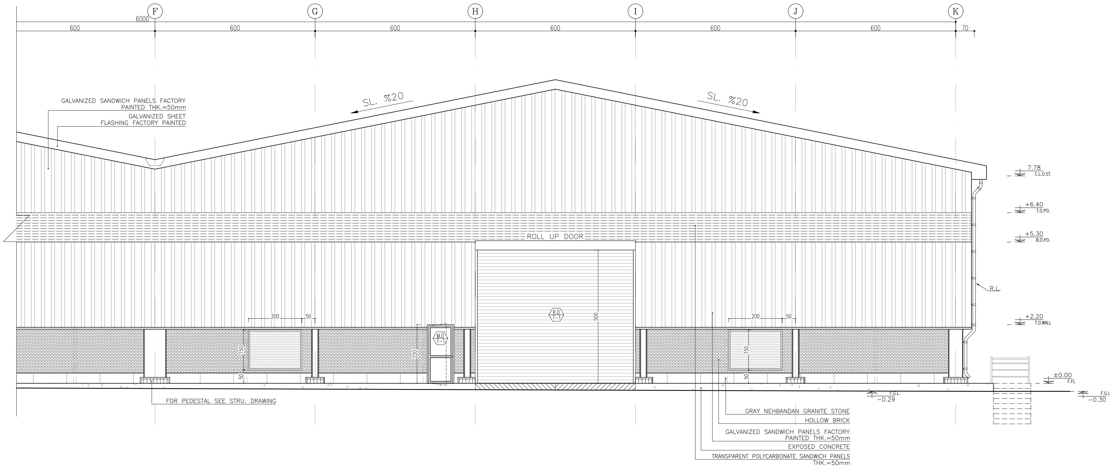
ELEVATION-1 Sc:1/75
