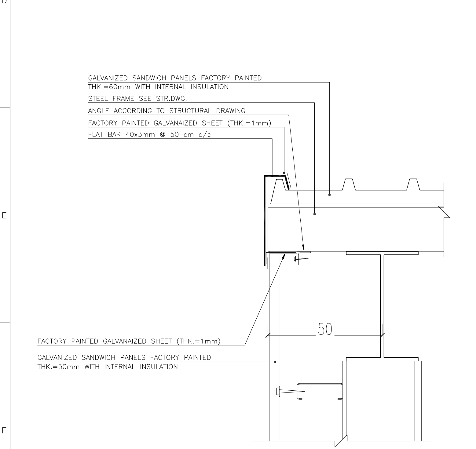
DETAIL-1 Sc:1/10
