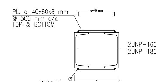
TYP. SECTION 2-2 Sc: 1:10
