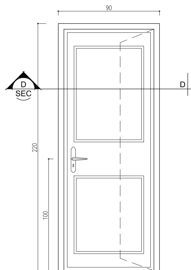
HDF DOOR – Type 1 NUMBER: 6 RIGHT HANDED: 2 LEFT HANDED: 4
