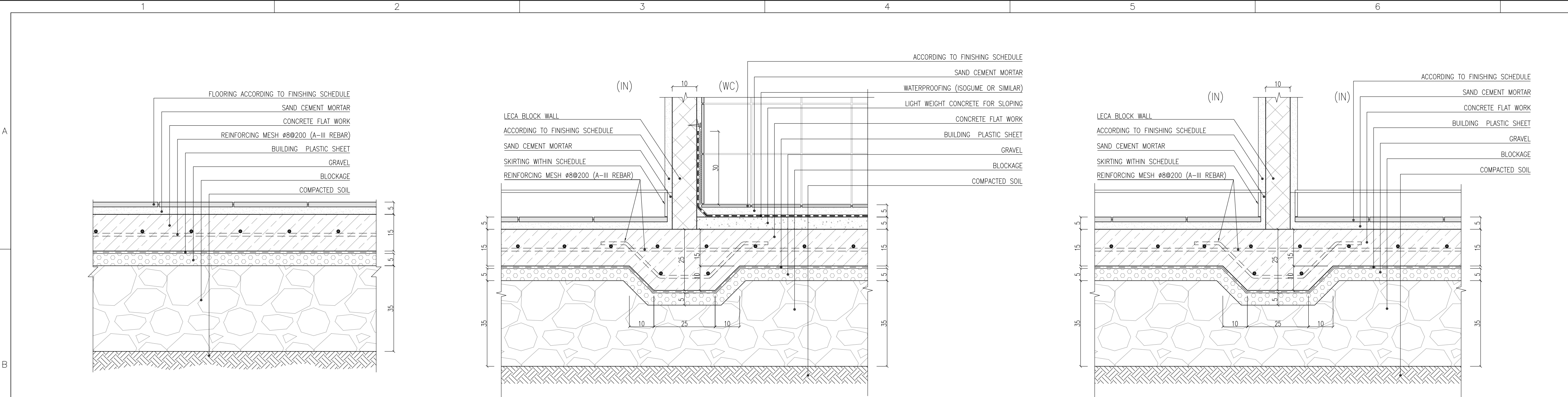
FLOORING DETAIL (GROUND FLOOR)
