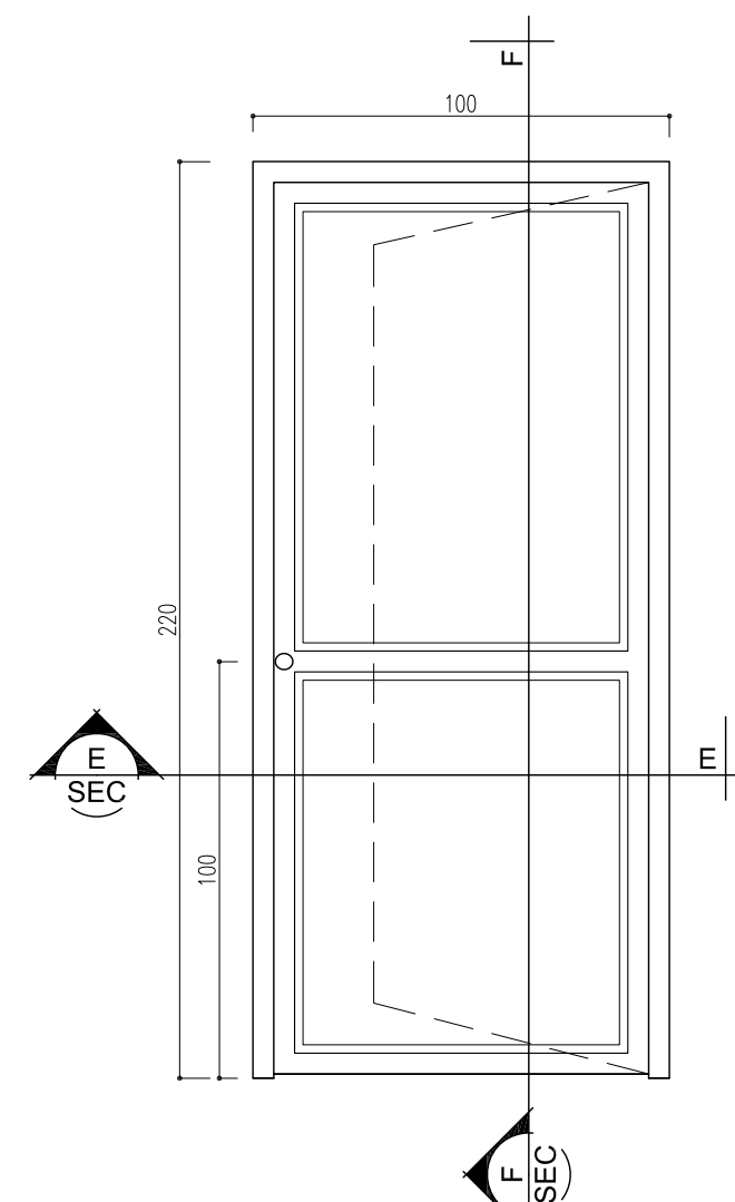
METAL DOOR - Type 1 NUMBER: 7 RIGHT HANDED: 3 LEFT HANDED: 4 Sc:1/20 M.D -1
