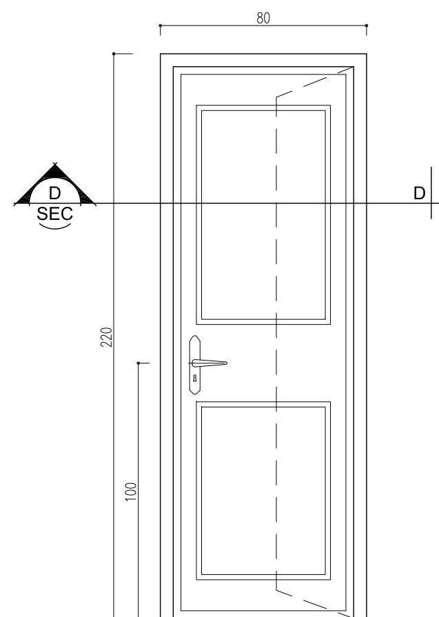
HDF DOOR – Type 2 NUMBER: 2 RIGHT HANDED: 2 LEFT HANDED: – Sc:1/20 HDF.D T-2
