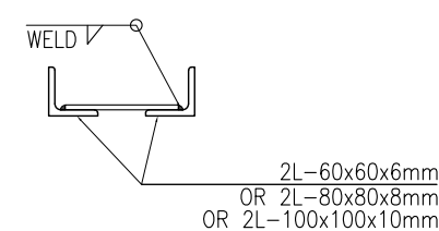
TYP. SECTION 1-1 Sc: 1:5
