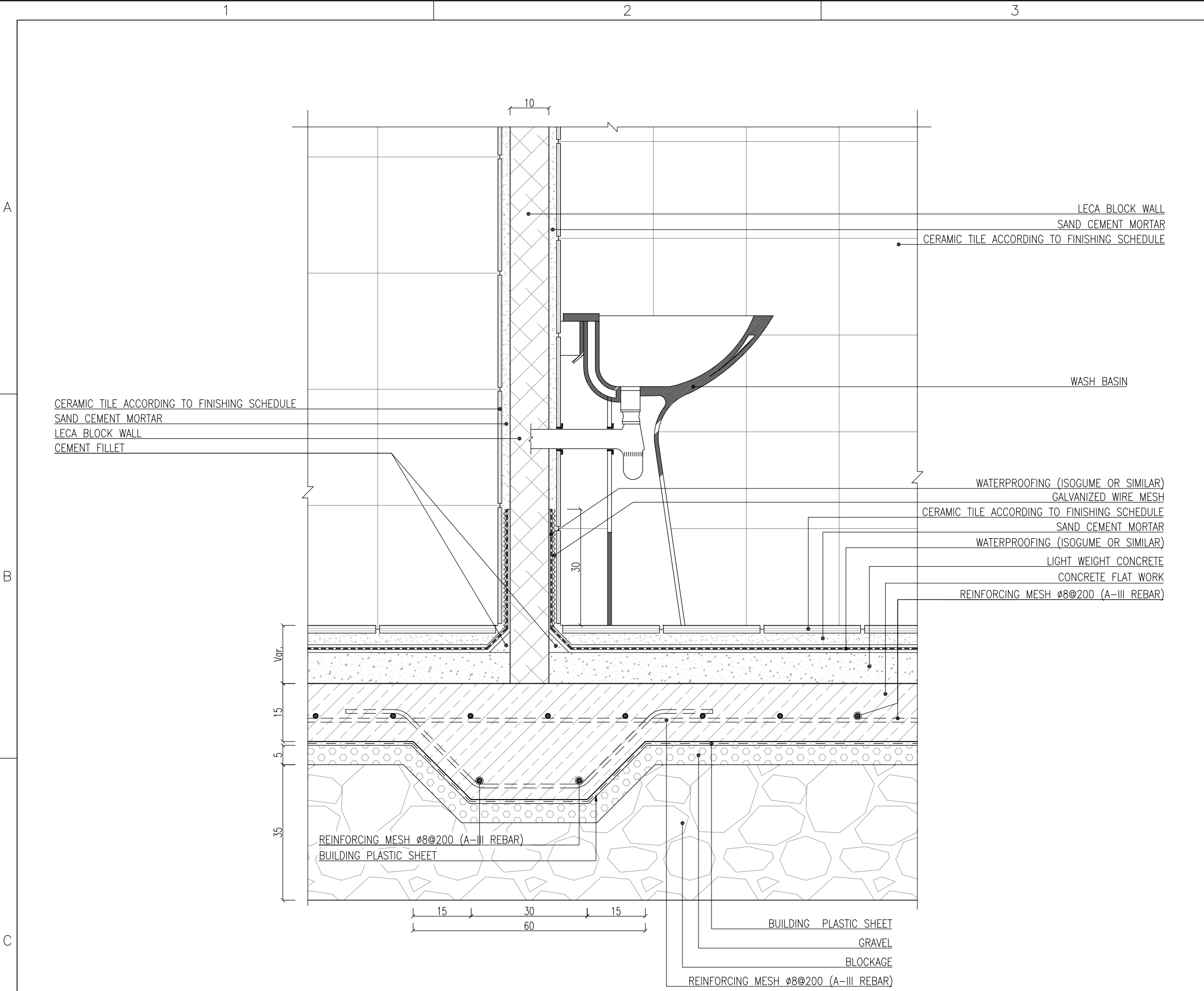
BASIN INSTALLATION DETAIL Sc:1/10
