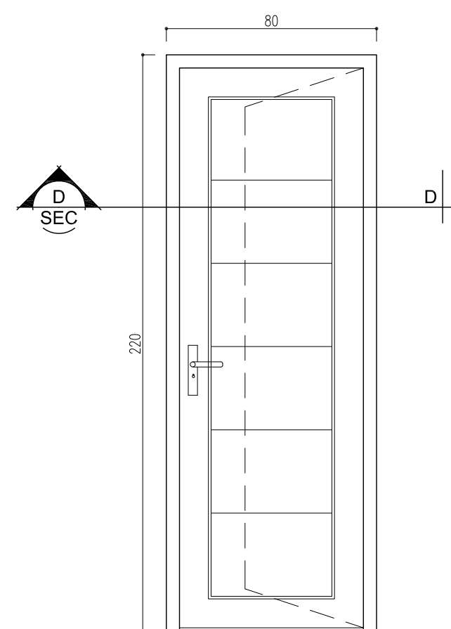
ABS DOOR – Type 1 NUMBER: 4 RIGHT HANDED: 1 LEFT HANDED: 3 Sc:1/20 ABS.D
