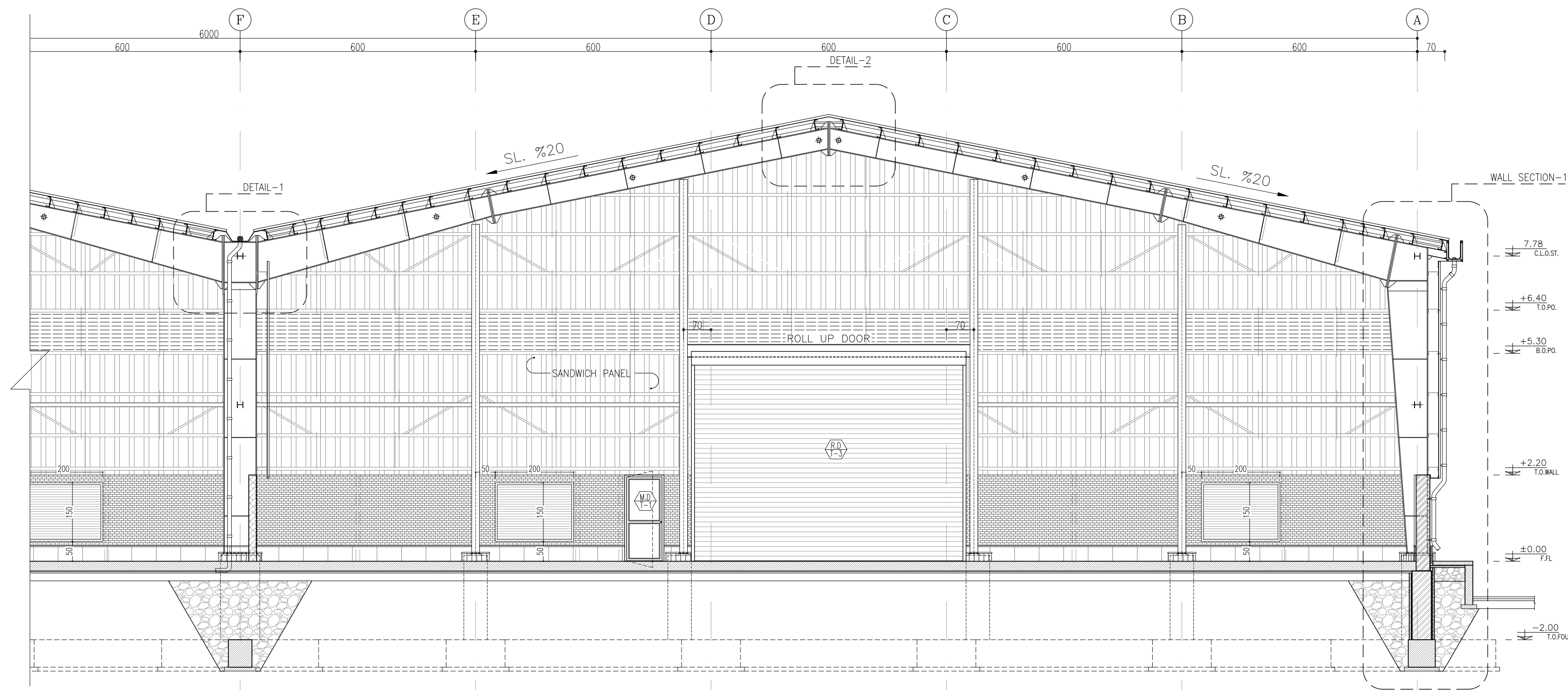
SECTION A-A Sc:1/75
