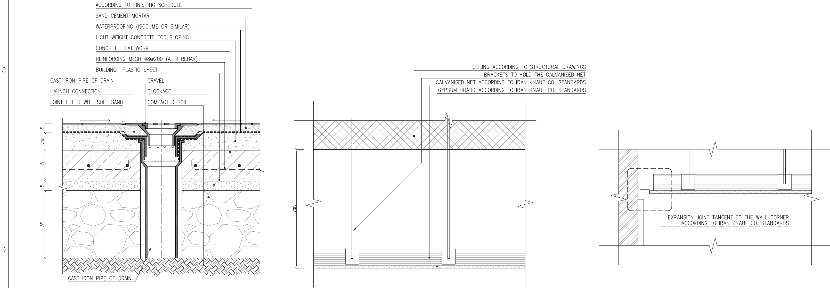
DRAIN DETAIL (GROUND FLOORS) Sc:1/10
