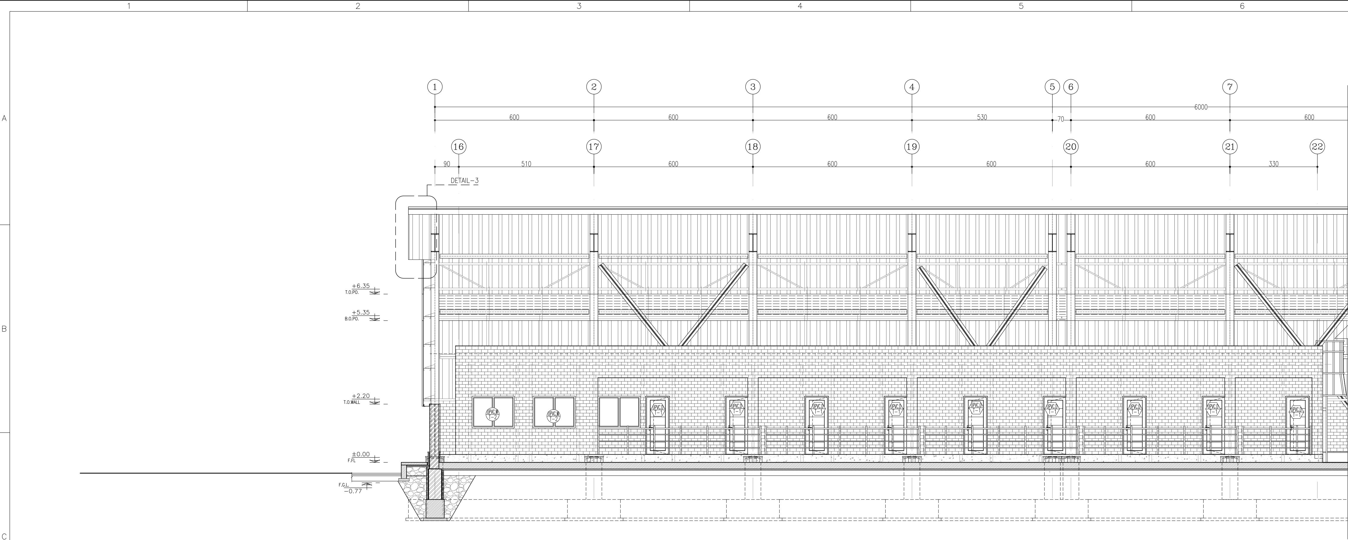
SECTION B-B Sc:1/75
