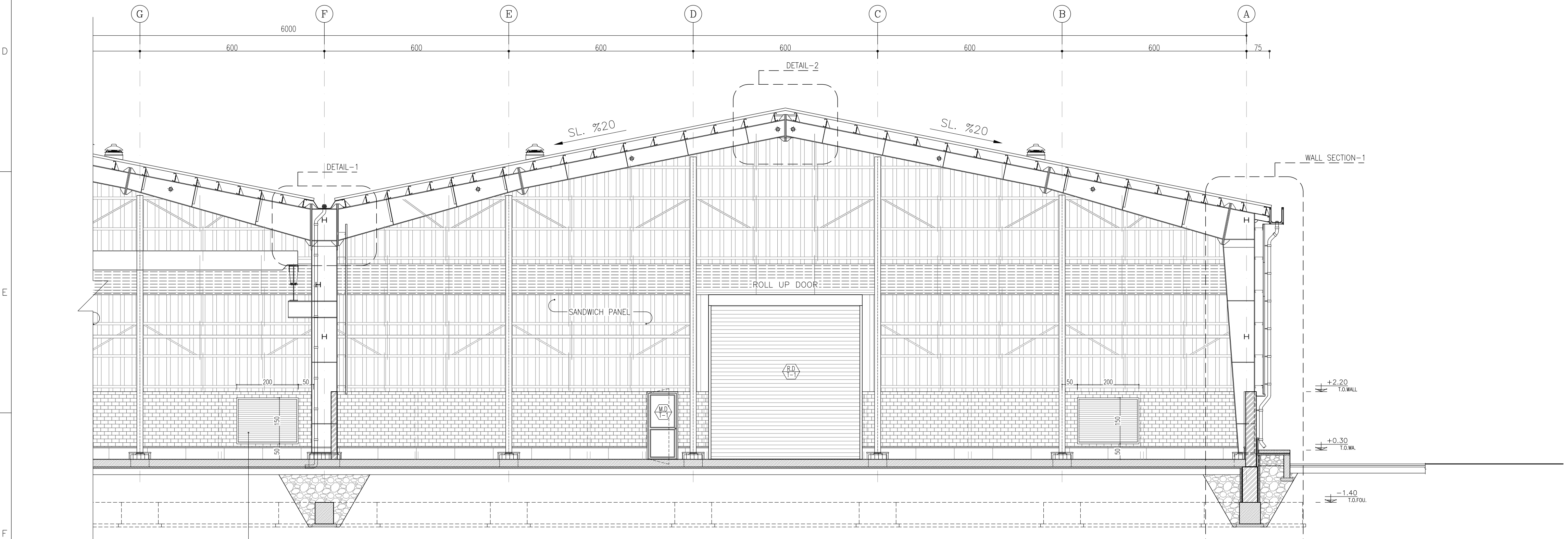
SECTION A-A Sc:1/75
