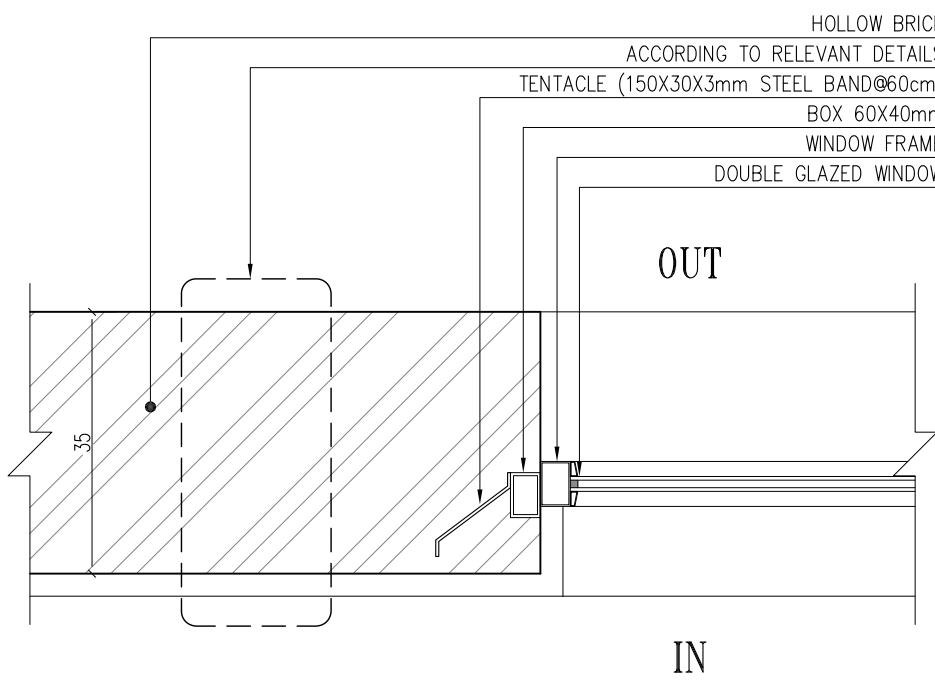
WINDOW LATERAL DETAIL Sc:1/10
