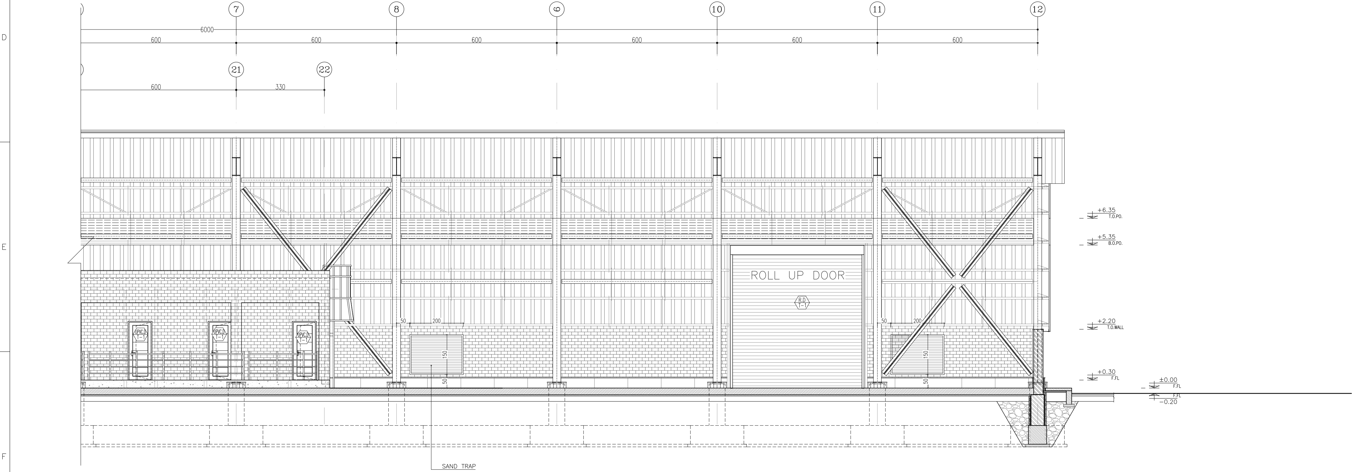
SECTION B-B Sc:1/75
