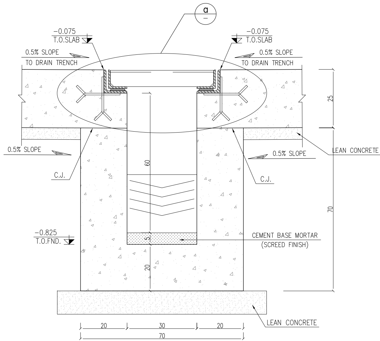
TYPICAL DETAILS FOR DRAIN TRENCH Sc:1/10
