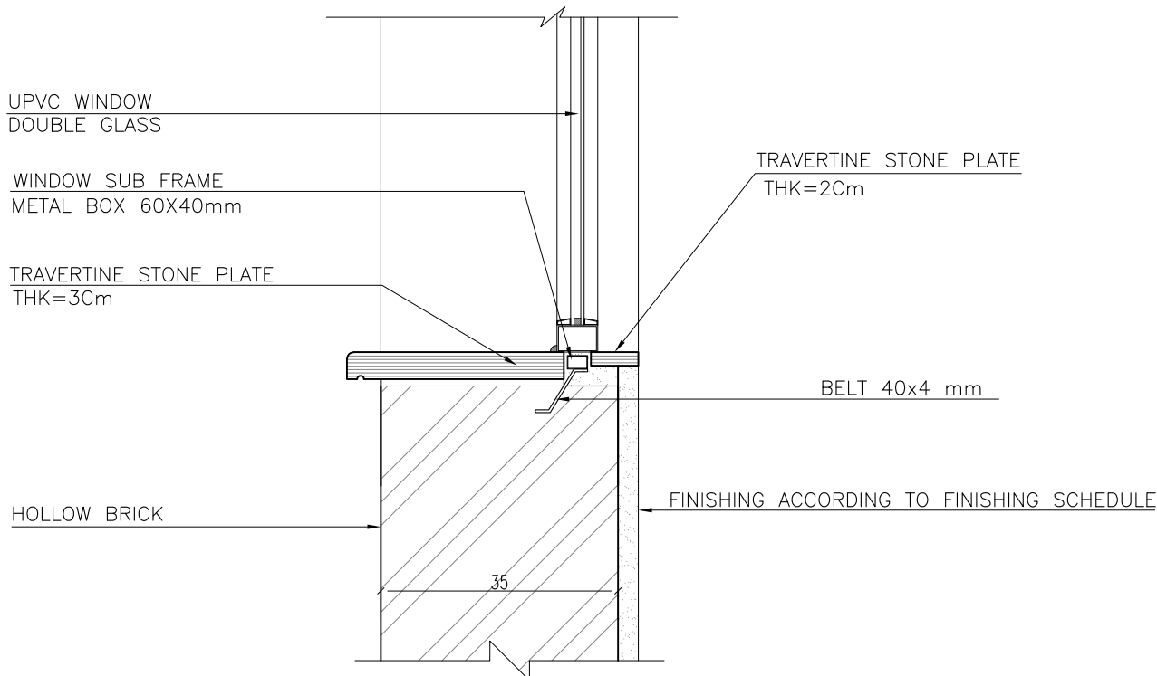
WINDOW SILL TYPICAL DETAIL Sc:1/10
