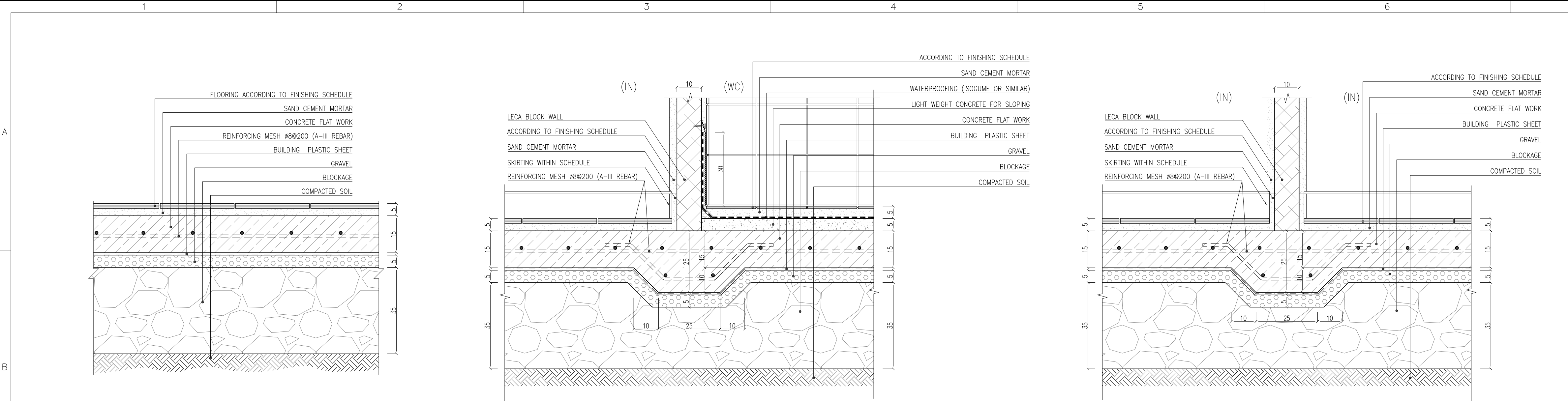
FLOORING DETAIL (GROUND FLOOR) Sc:1/10
